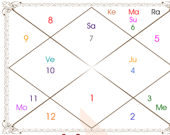
Shodasamsa Chart
