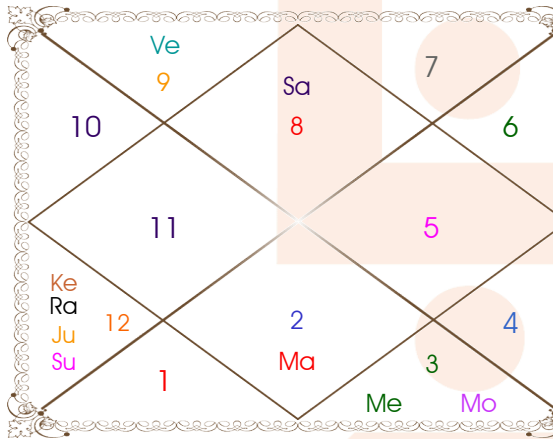
Trimsamsa Chart
