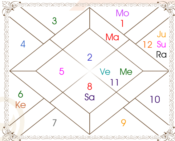
Chalit Chart
