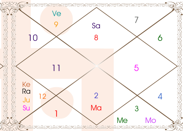
Trimsamsa Chart
