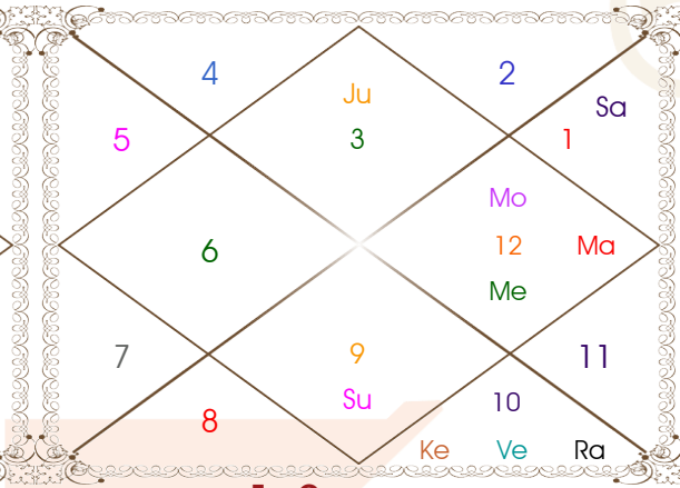
Shodasamsa Chart
