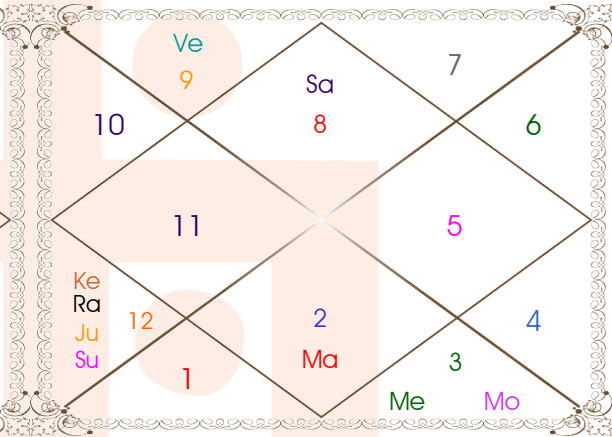
Trimsamsa Chart
