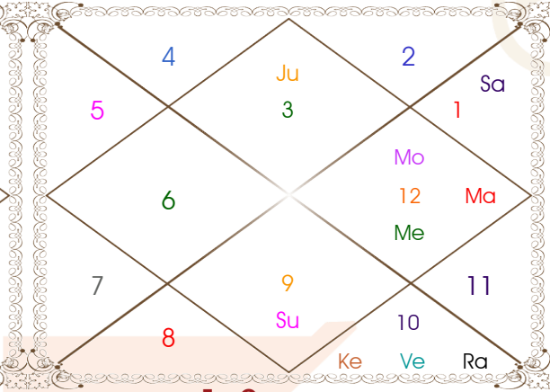
Shodasamsa Chart
