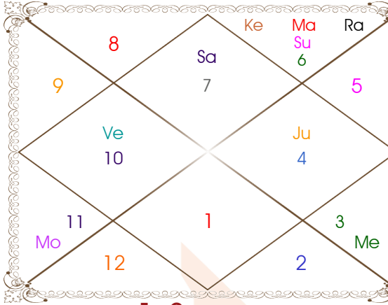
Shodasamsa Chart
