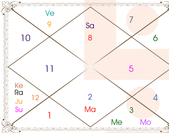
Trimsamsa Chart
